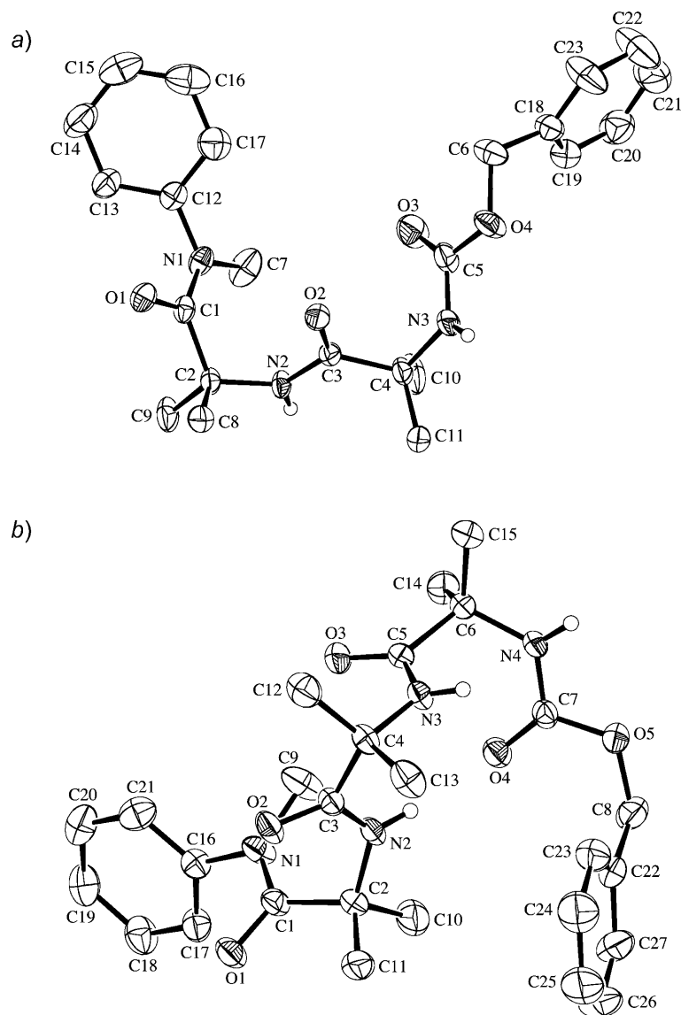
Fig. 1. ORTEP Plots [19] of the molecular structures of a) 6a and b) one of the two symmetry-independent molecules of 8a (50% probability ellipsoids, arbitrary numbering of the atoms)
