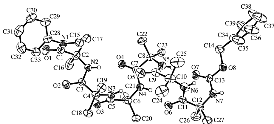
Fig. 3. ORTEP Plot [19] of the molecular structure of 14 (50% probability ellipsoids, arbitrary numbering of the atoms, the H 2 O molecule has been omitted)
