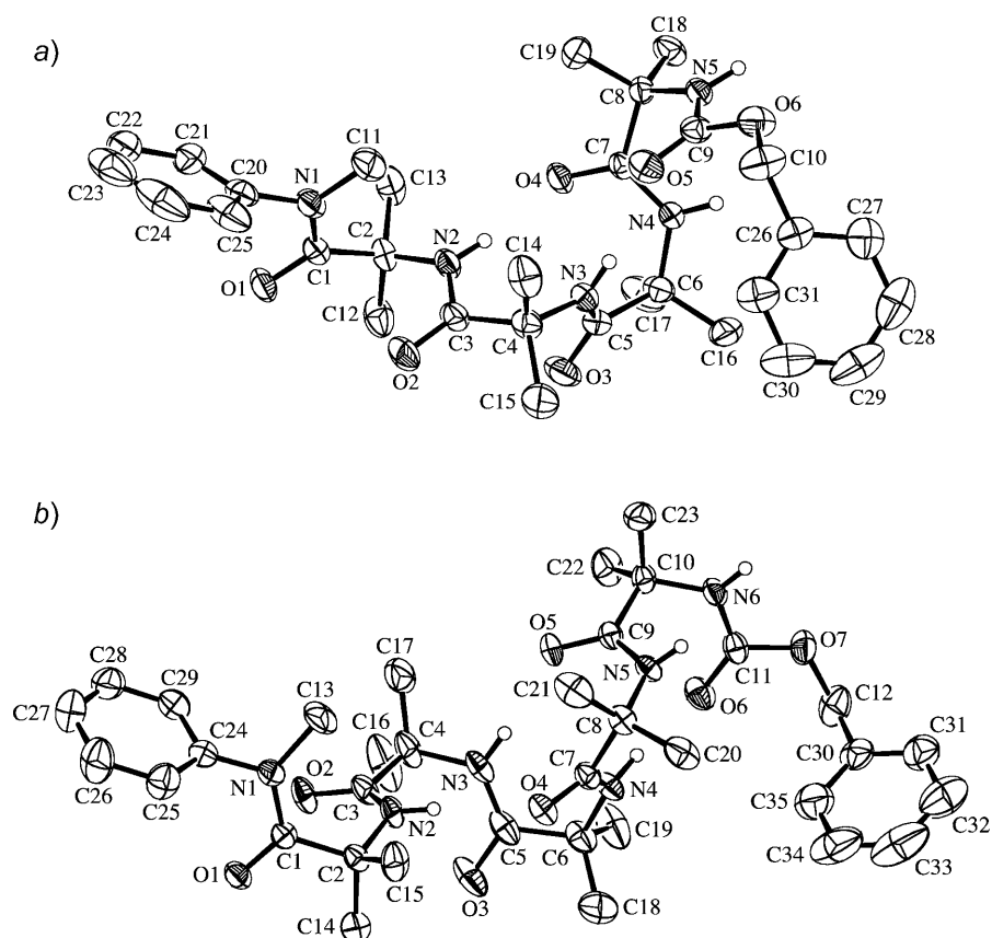
Fig. 2. ORTEP Plots [19] of the molecular structures of a) 10 and b) 12 (50% probability ellipsoids, arbitrary numbering of the atoms, H 2 O molecule in 10 omitted)
